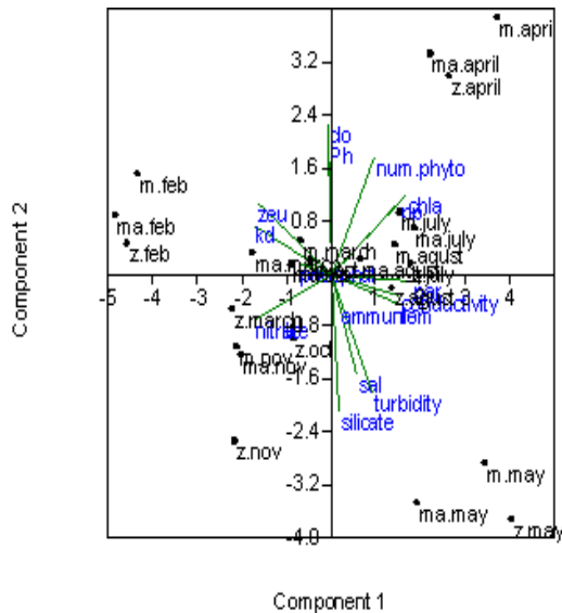
Figure 6: Biplot based on Principal Component Analysis (PCA) of chlorophyll- a , primary production and 12 environmental parameters for 3 stations for the period Feb 2014 till Nov 2014 along Khuzestan’s waters (ma: Mahshahr Creek, m: Moussa Creek and z: Zangi Creek).
