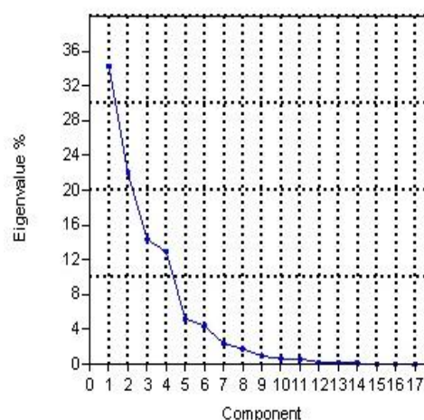
Figure 5: Scree plot of the eigenvalues in the northwest Persian Gulf.
