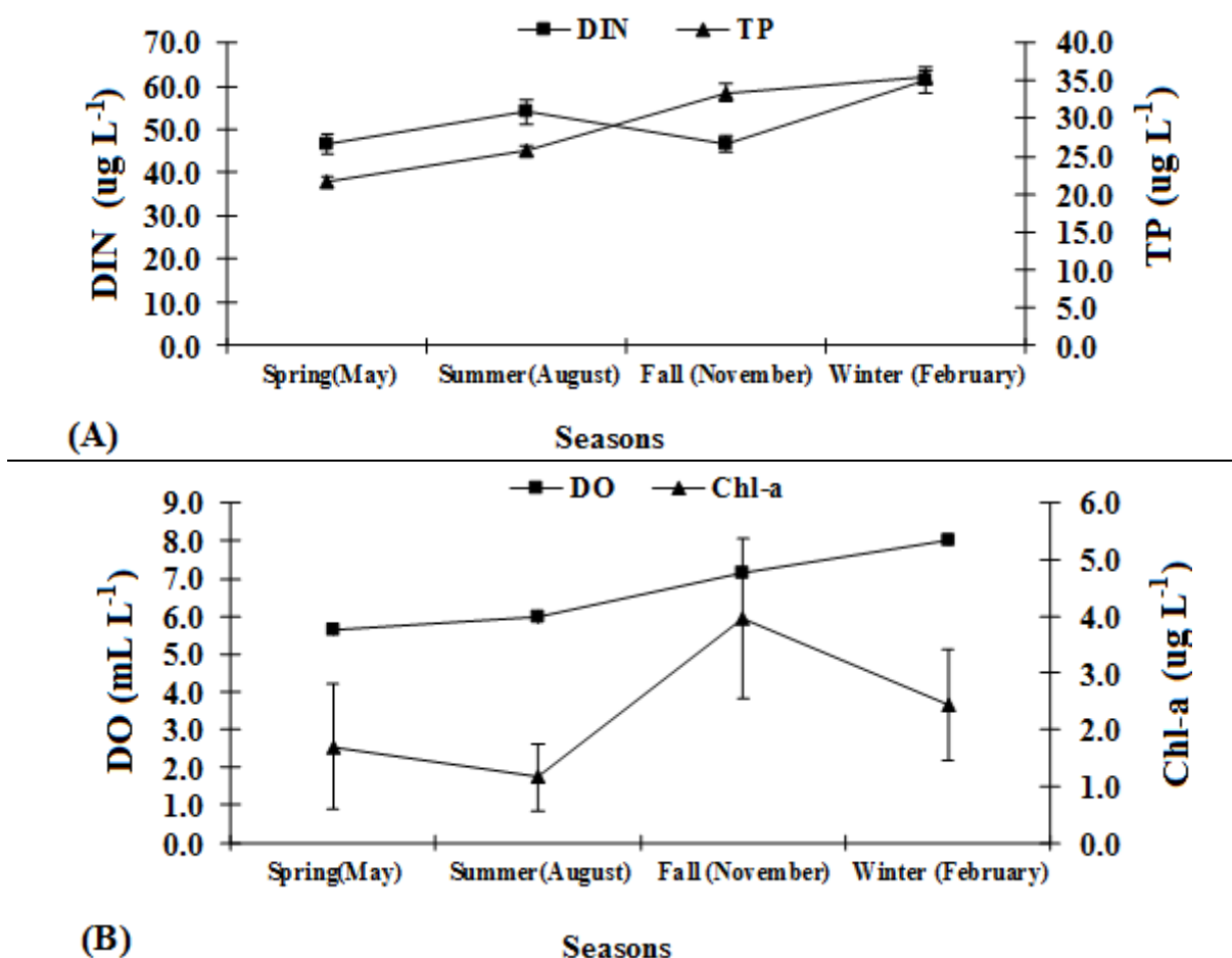
Figure 2: Seasonal changes in the mean concentrations of environmental parameters collected from four transects in ICWCS (2013-2014). (A) DIN and TP; (B) DO and Chl-a.
