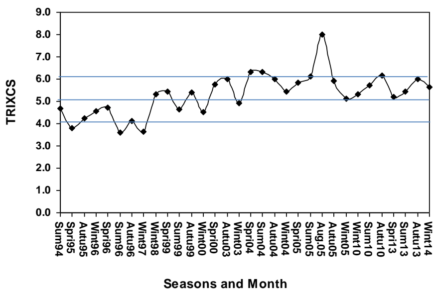
Figure 3: Long-term changes in the trophic index of ICWCS based on TRIX CS values. Long term data was adopted from Nasrollahzadeh Saravi (2008). The data for August 2005 was adopted from Soloviev (2005). Note the high peak of TRIX CS was in August 2005 when one species of Cyanophyta bloomed in the area.
